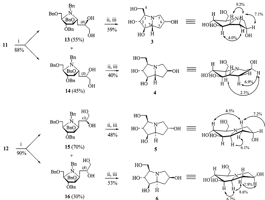
Scheme 3. Reagents and conditions: (i) cat. OsO 4 , NMO, acetone/water; (ii) TsCl, Py; (iii) 10% Pd/C, HCO 2 NH 4 , MeOH, 60 °C
