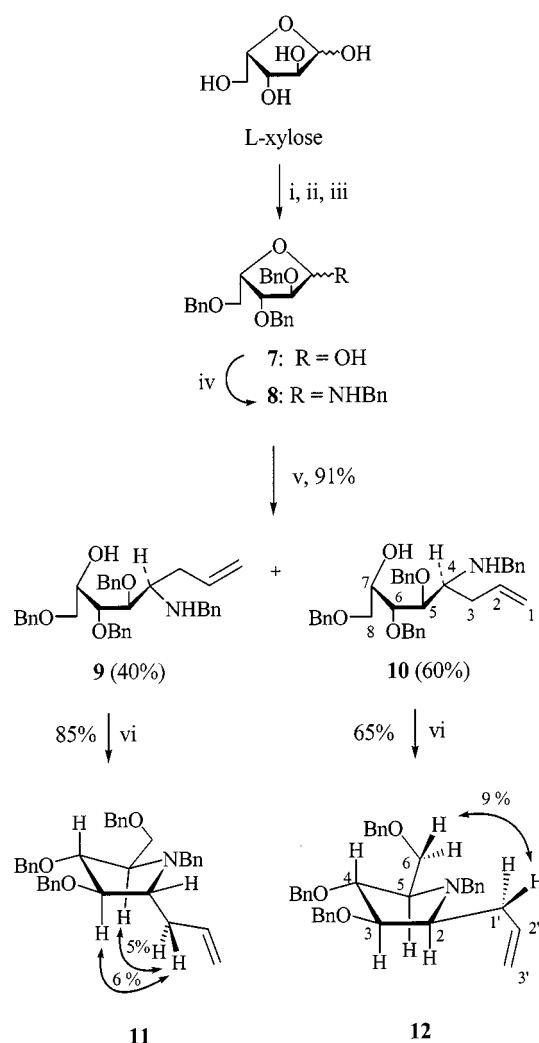
Scheme 2. Reagents and conditions: (i) MeOH/HCl, 100%; (ii) BnBr, Ba(OH) 2 , DMF, 40%; (iii) aq. HCl, refluxing dioxane, 50%; (iv) BnNH 2 , CH 2 Cl 2 , mol. sieves (4 Å), 98%; (v) allylMgCl, THF, 0 °C; (vi) MsCl, Py
